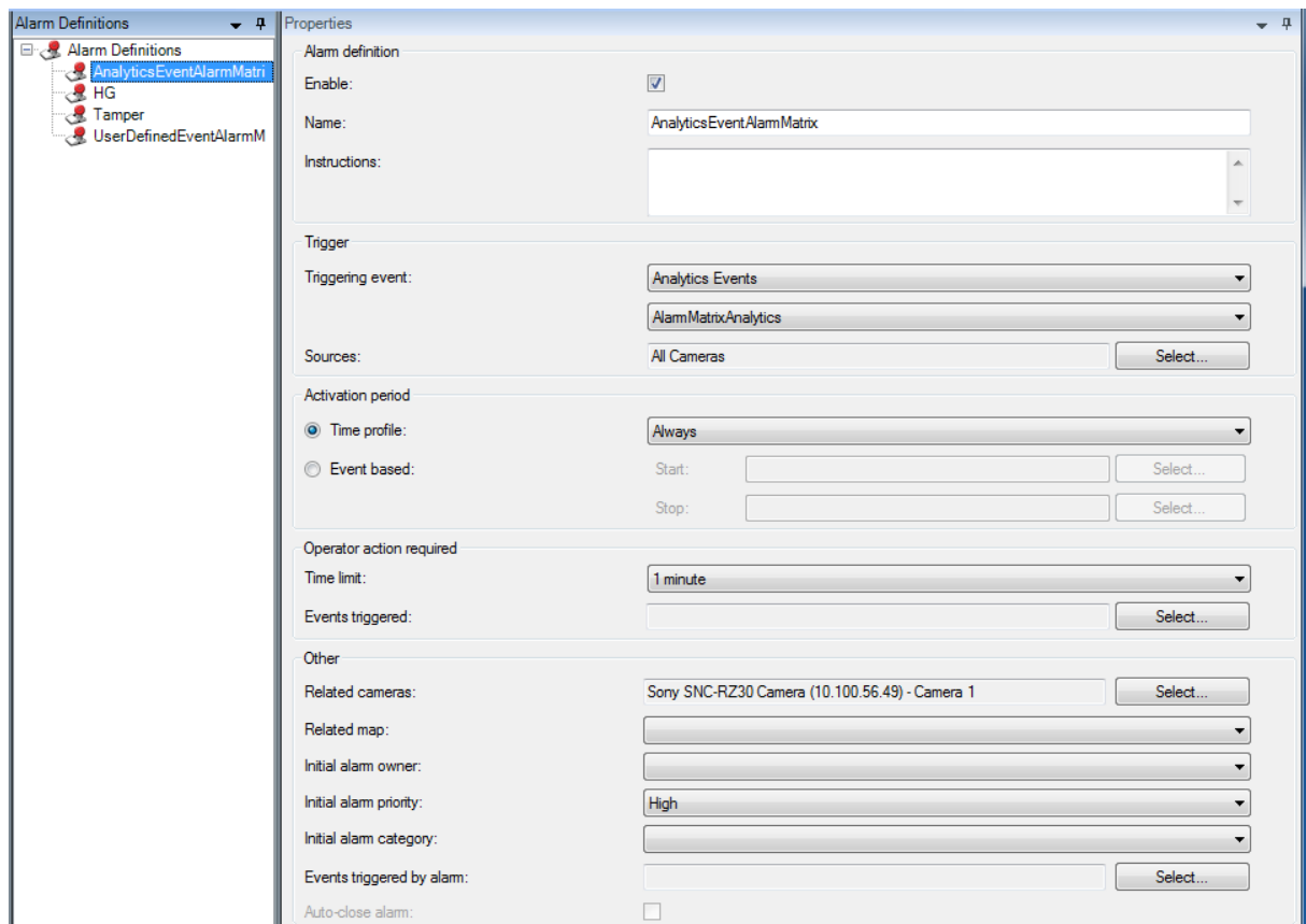
Figure 10: Defining a new user defined alarm for Alarm Matrix
